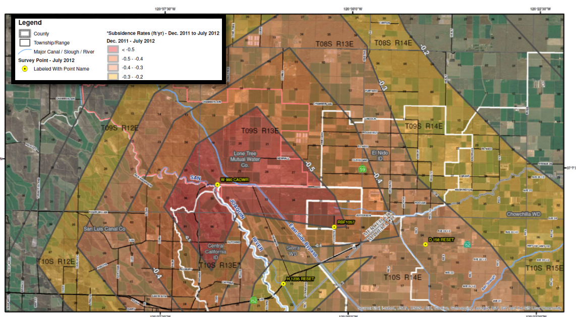
Figure 4-4. Subsidence Rates in the Washington Avenue/Red Top Areas
