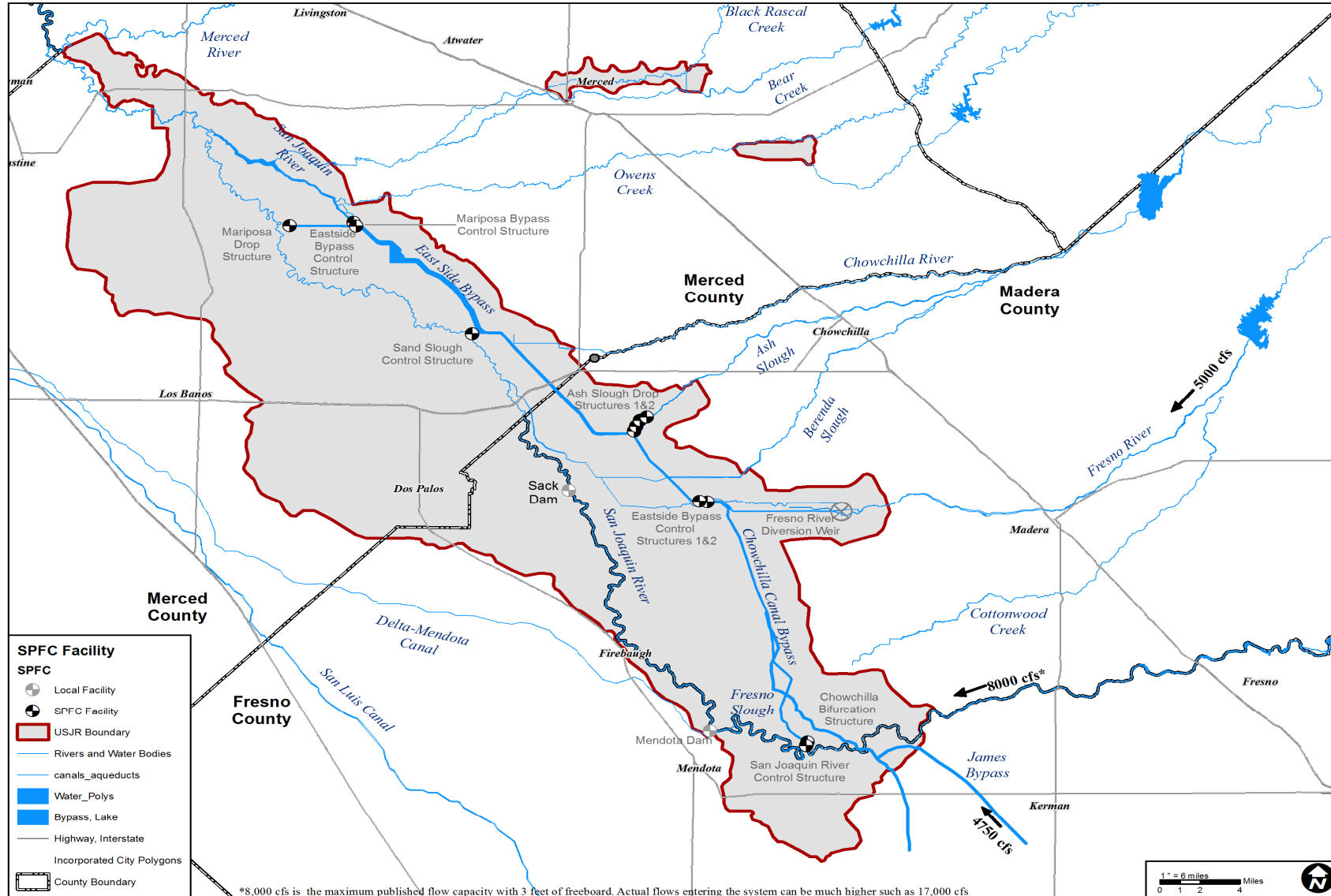
Figure 4-3. Location and Amount of Published Maximum Upstream Design Flow Capacity
