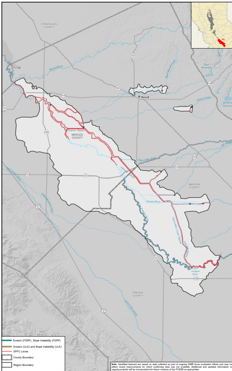
Figure 4-7. Slope Instability and Erosion Locations in the USJR Region
