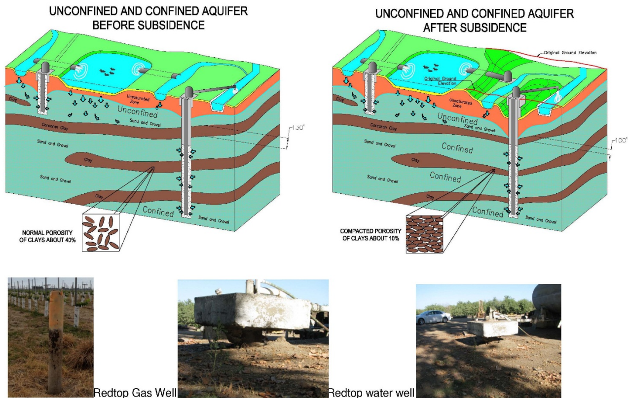
Figure 4-5. Cross Section Demonstrating Effects of Subsidence and Photos of Subsidence
