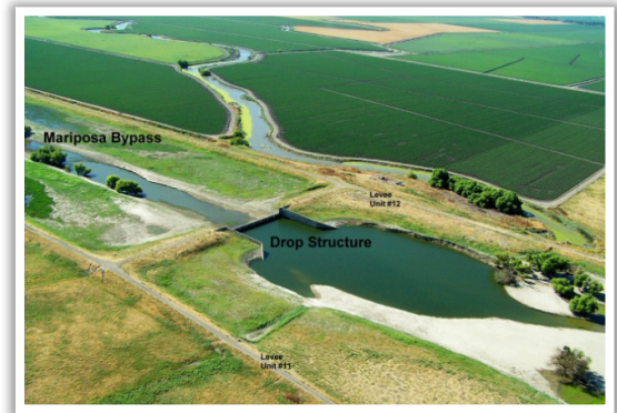
Mariposa Bypass Control Structure
