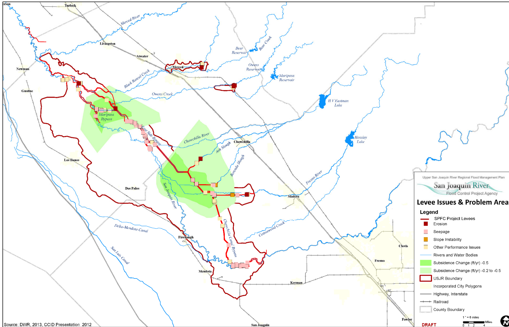
Figure 4-2. Levee Issues and Problem Areas
