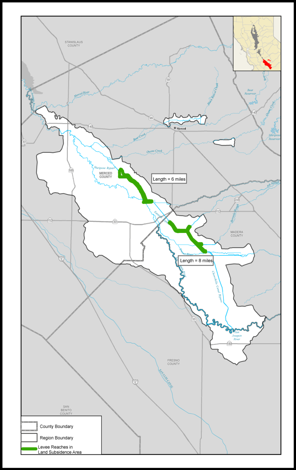
Figure 4-6. Areas of Subsidence in the USJR Region
